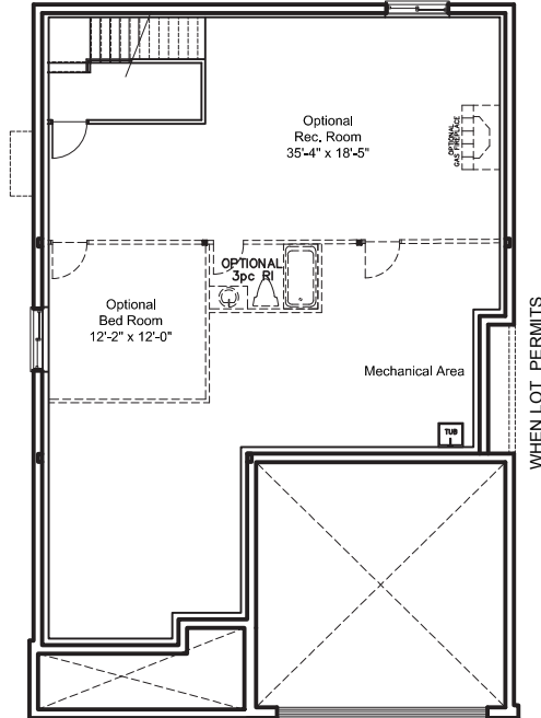
BASEMENT FLOOR - ELEVATION A & C
