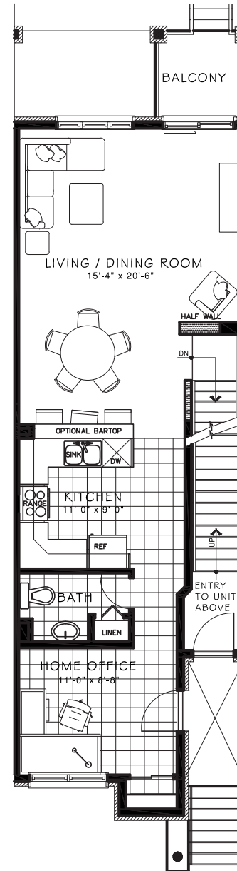
1ST FLOOR MID UNIT - MODEL 2100
