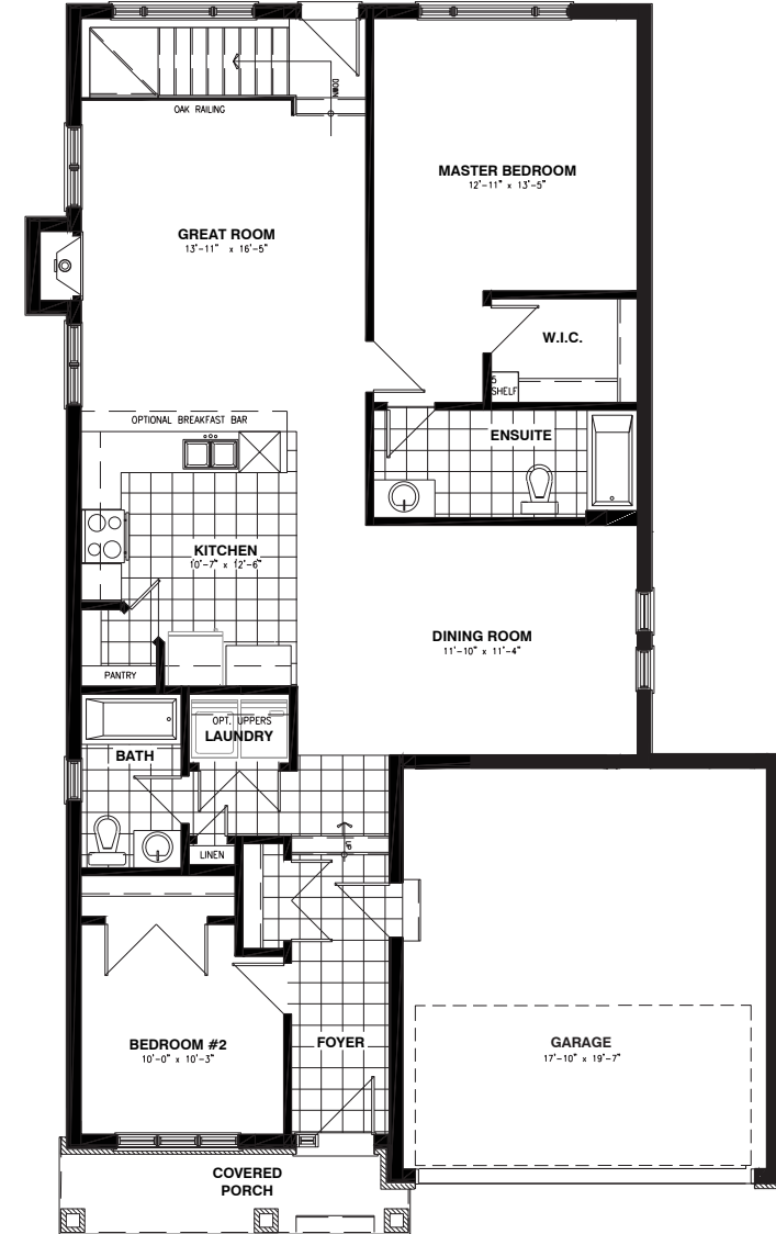
GROUND FLOOR A
