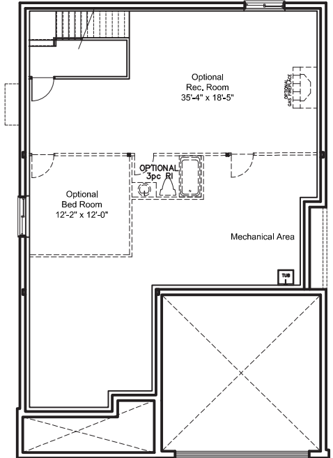
BASEMENT FLOOR - ELEVATION A & C
