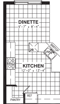
OPTIONAL KITCHEN #1
