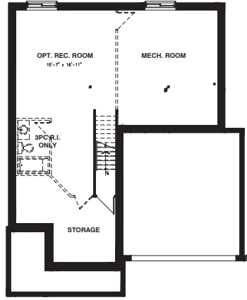
BASEMENT FLOOR ELEVATION A
