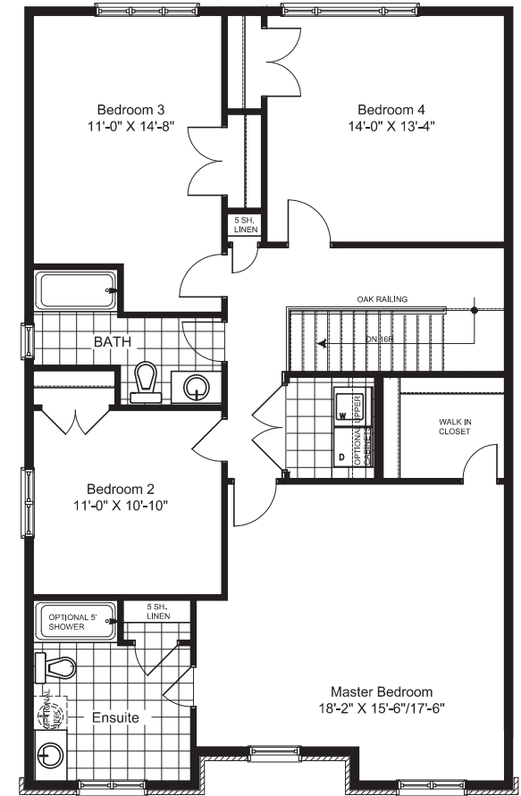
SECOND FLOOR - 4 BEDROOMS - ELEVATION A
