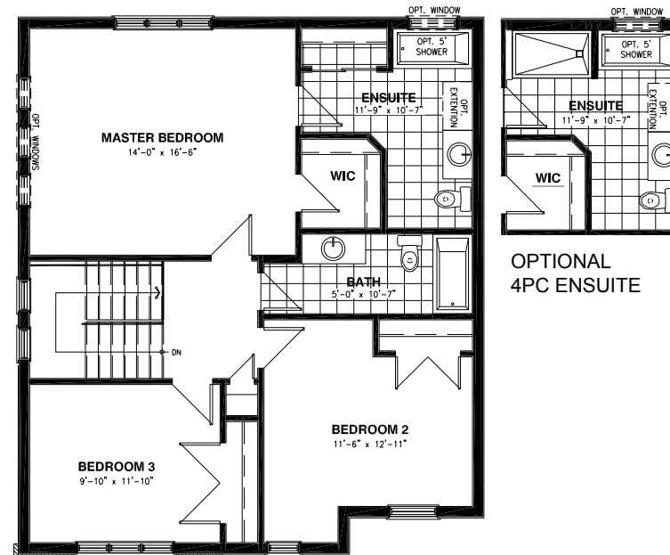
SECOND FLOOR - 3 BEDROOMS ELEVATION A
