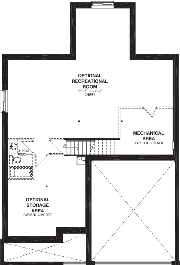
BASEMENT FLOOR
