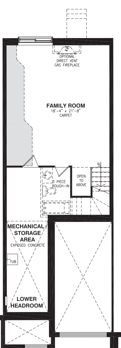
BASEMENT FLOOR
