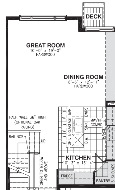
OPTIONAL KITCHEN #1
