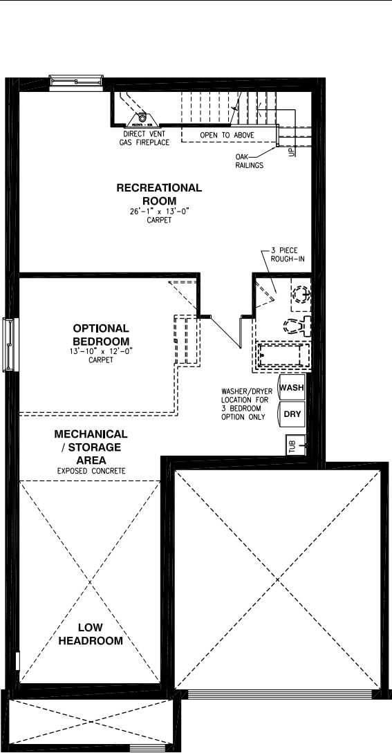
BASEMENT FLOOR
