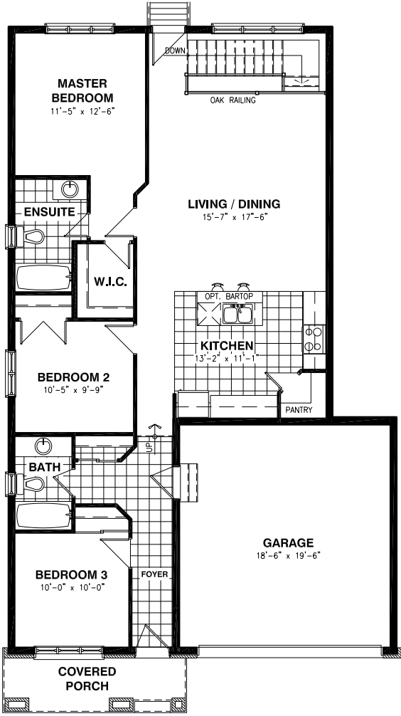
STANDARD 3 BEDROOMS GROUND FLOOR ELEVATION A
