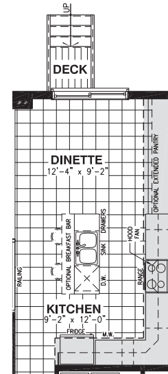
OPTIONAL KITCHEN #1
