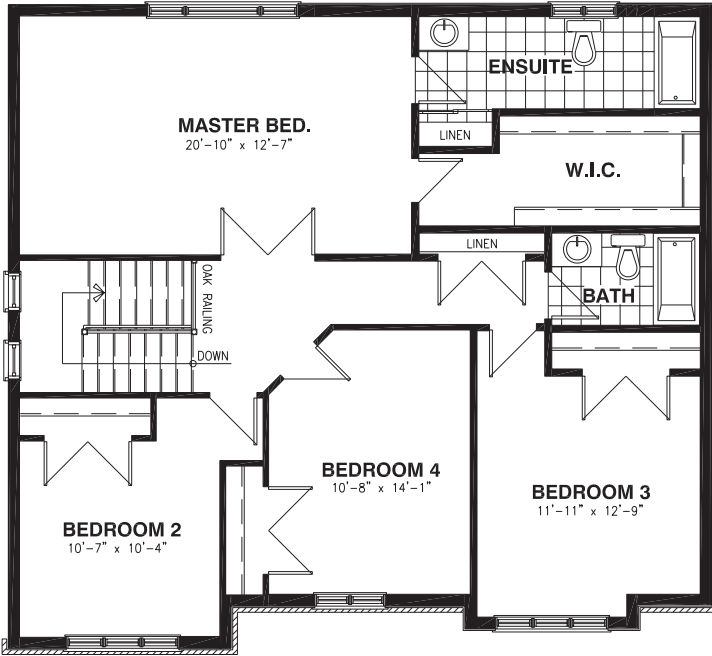
SECOND FLOOR - ELEVATION A
