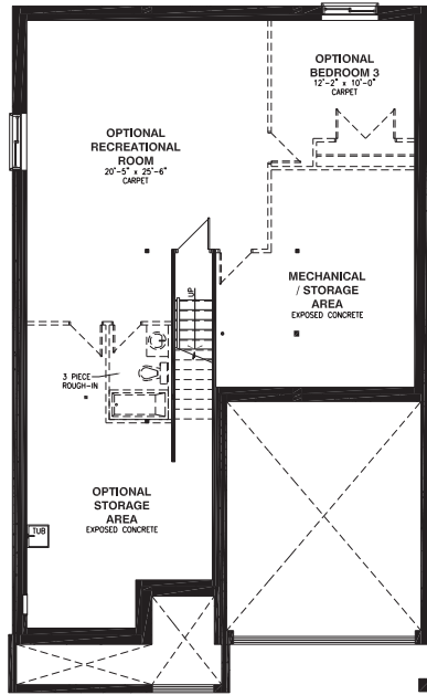
BASEMENT FLOOR - ELEVATION LOFT
