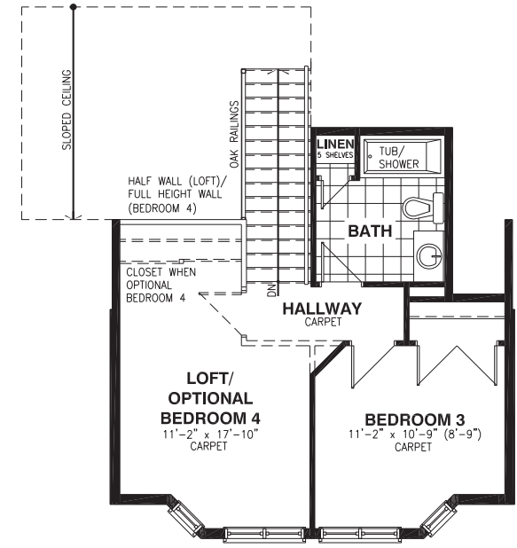
SECOND FLOOR - ELEVATION LOFT
