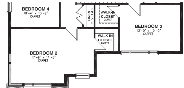
SECOND FLOOR - ELEVATION B
