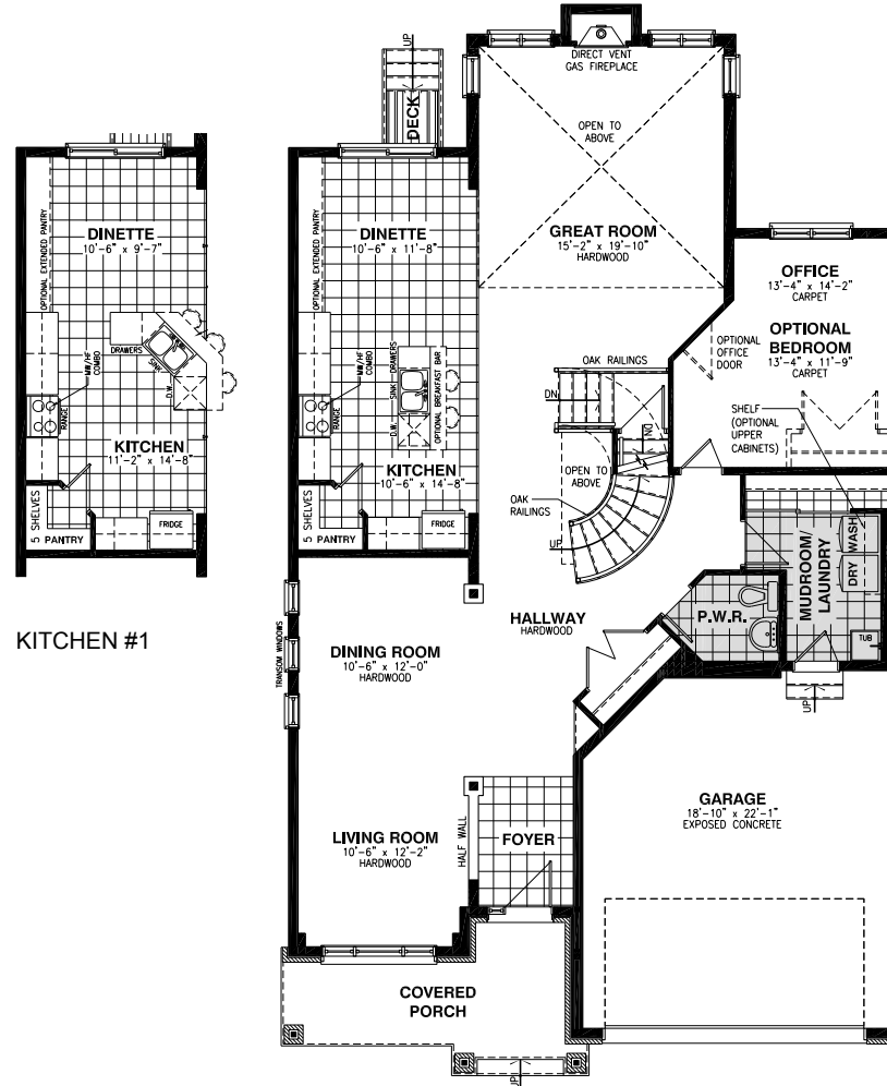
GROUND FLOOR - ELEVATION A
