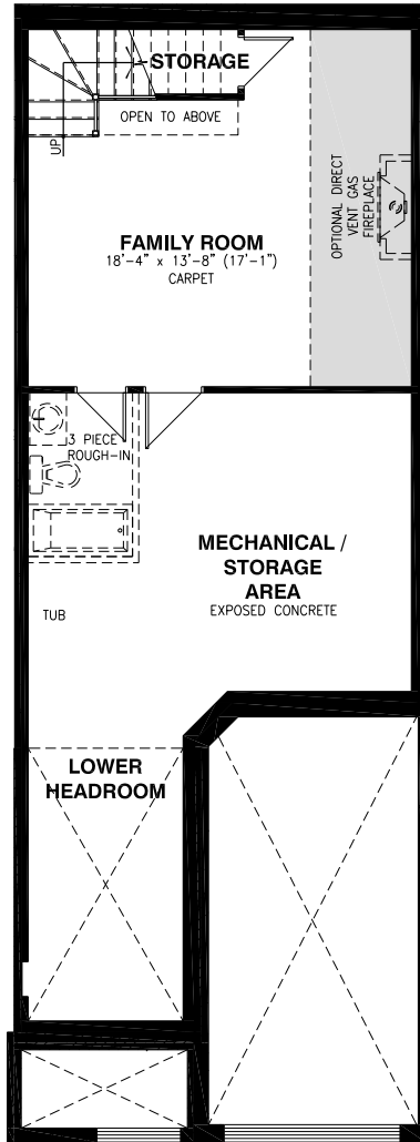
BASEMENT FLOOR
