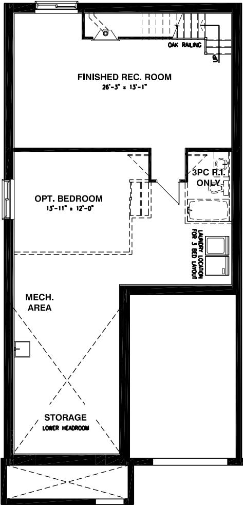
BASEMENT FLOOR
