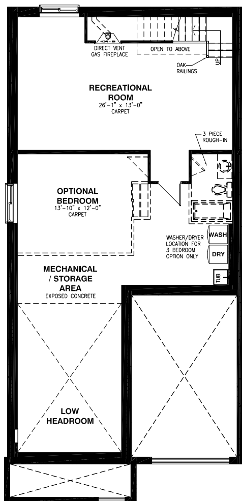
BASEMENT FLOOR
