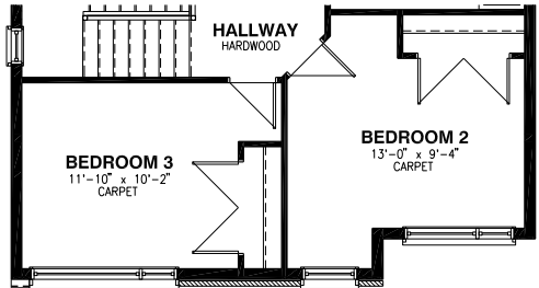
SECOND FLOOR - 3 BEDROOMS ELEVATION B
