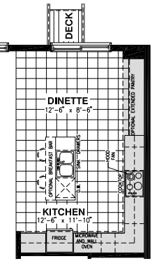
OPTIONAL KITCHEN #3
