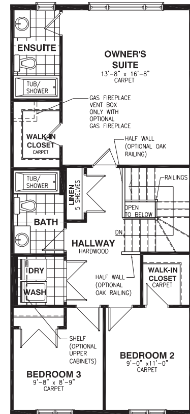
SECOND FLOOR
