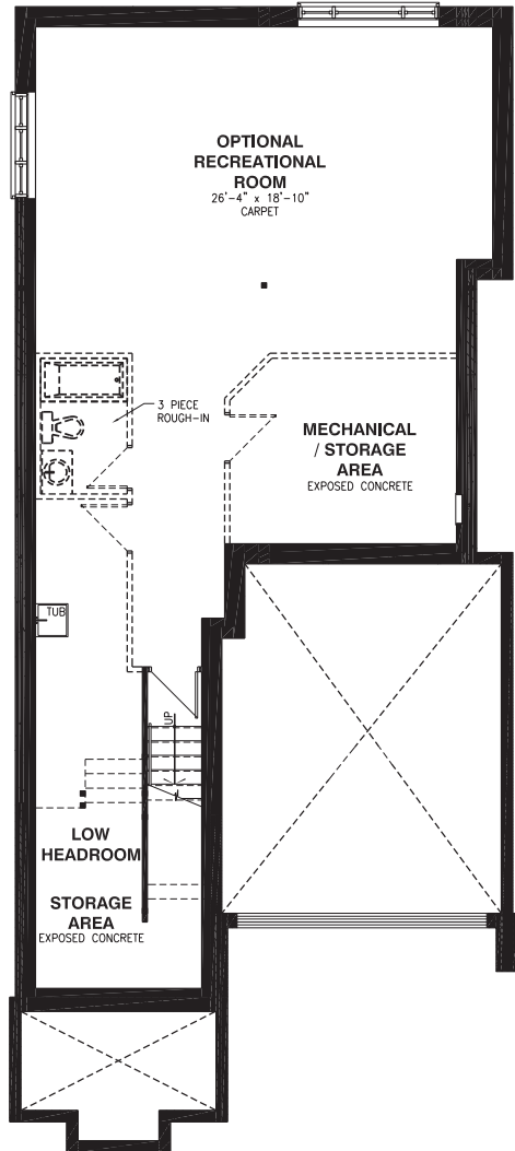
BASEMENT FLOOR - ELEVATION A
