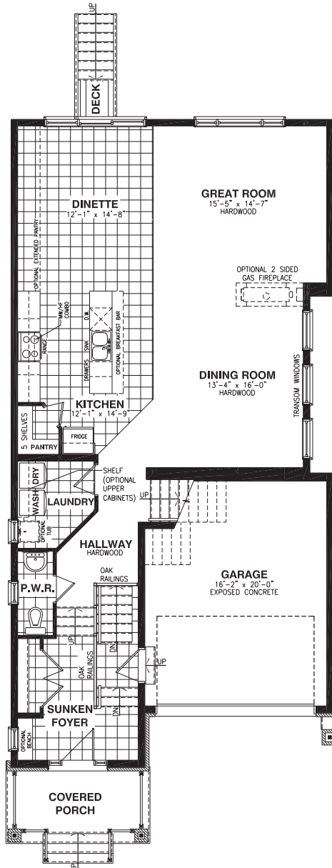
GROUND FLOOR - ELEVATION A
