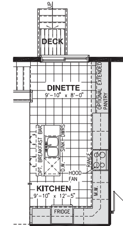
OPTIONAL KITCHEN #2
