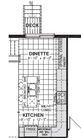
OPTIONAL KITCHEN #3
