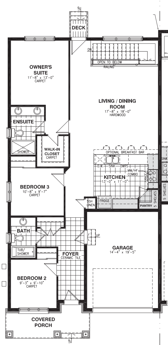
GROUND FLOOR - STANDARD 3 BEDROOMS
