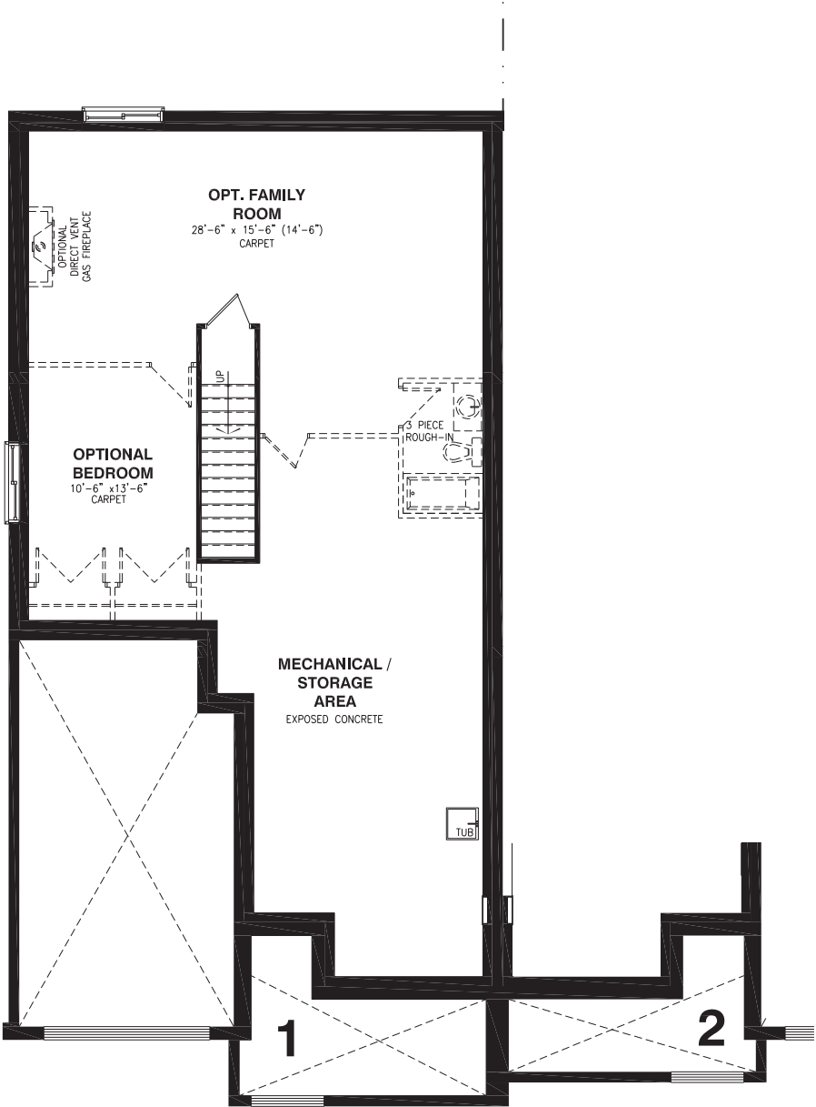
BASEMENT FLOOR
