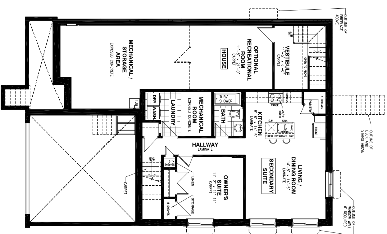
Basement Floor - Elevation A
