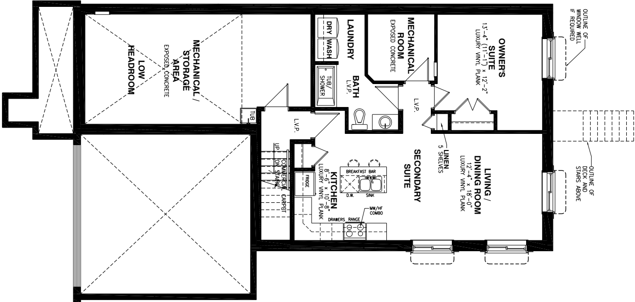
Basement Floor - Elevation A and B
